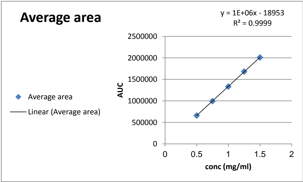
Figure 3.11. Calibration curve of amlodipine in plasma
